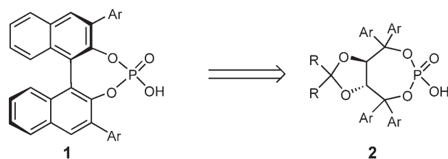
Figure 1. Plausible transition state.
