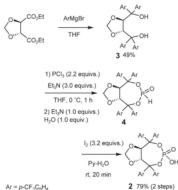
Scheme 1. Preparation of chiral catalysts; yields are given for Ar = p -CF 3 C 6 H 4 .
